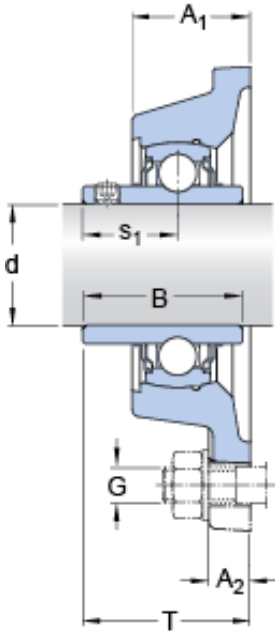
FY 1.15/16 TF/VA228 Bearing 2D drawings and 3D CAD models
